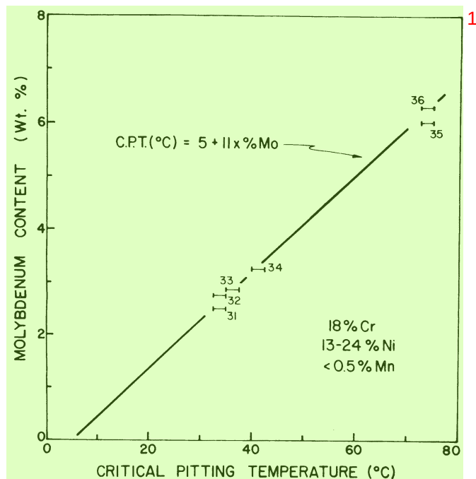
FIGURE 6 — Critical pitting temperature as a function of molybdenum content for a family of low (<0.5%) Mn stainless steels which exhibit superior pit initiation resistance. The numbers refer to alloys listed in Table 1.
