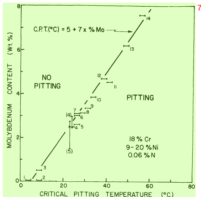
FIGURE 3 – Critical pitting temperature as a function of molybdenum content for an average family of 18% Cr, low nitrogen, experimental and commercial stainless steels which are representative of steels made by present commercial practice. Unbracketed numbers refer to alloys listed in Table 1. Bracketed numbers refer to data cited in the literature.
