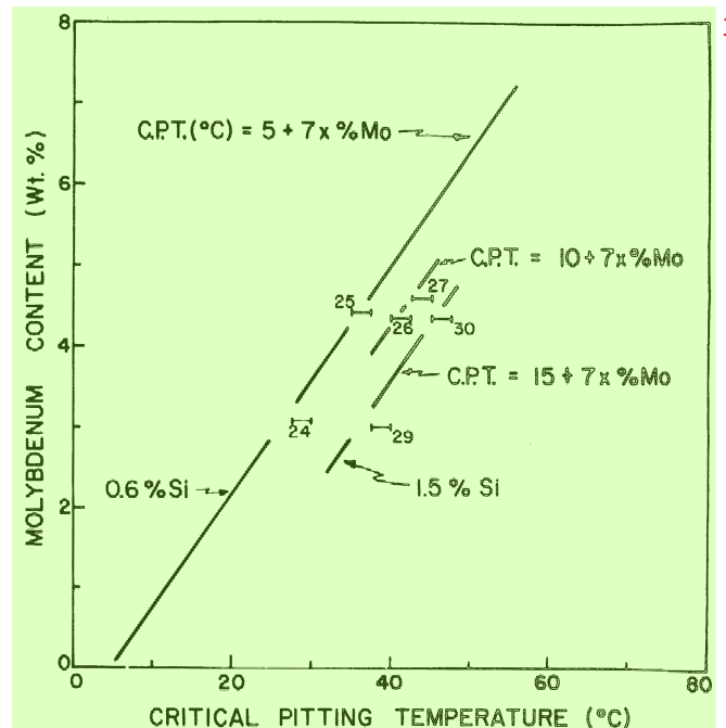
FIGURE 5 – Critical pitting temperature as a function of molybdenum content for three families of austenitic stainless steels showing the effect of increasing Si content. The numbers refer to alloys listed in Table 1. Alloys 24, 25, and 26 contain alloyed Cu but fall in the same families as other similar steels which do not contain Cu.
