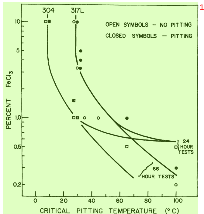
FIGURE 2 – Critical pitting temperature of 304 and 317L stainless steels as a function of \text{FeCl}_3 concentration in 24 and 66 hour tests.
