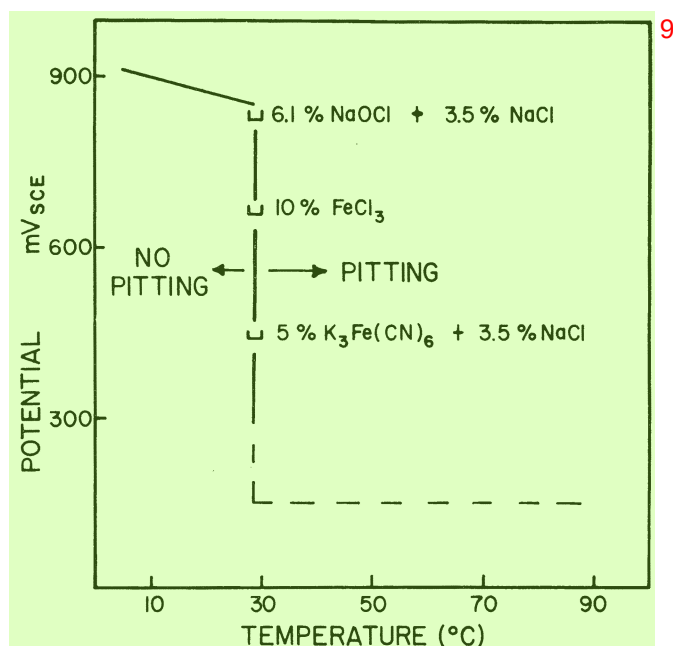
FIGURE 1 — Pitting temperature range of 317L austenitic stainless steel tested in chloride solutions of different oxidizing power (potential) for 24 and 66 hours. Dashed portion of the curve is based on potentiodynamic polarization data. 1 9
